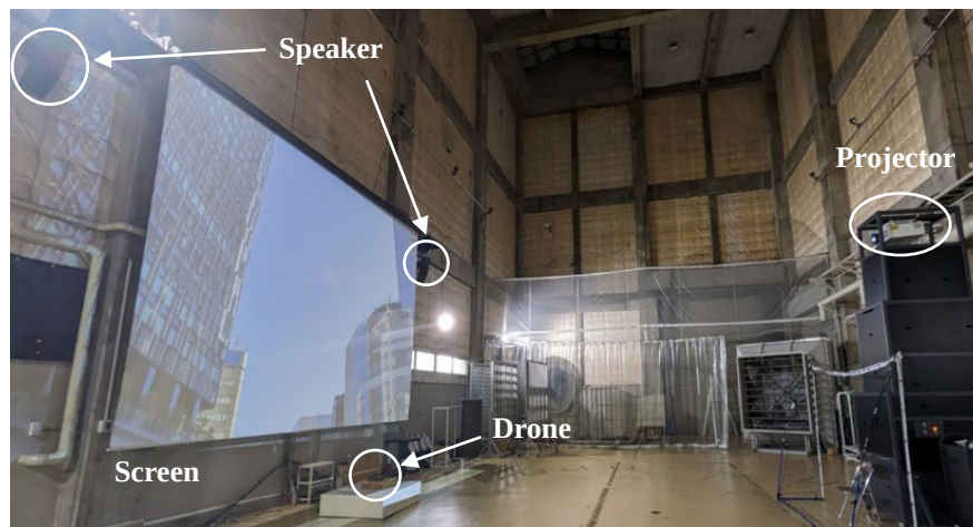
Fig.5 Experiment environment.
