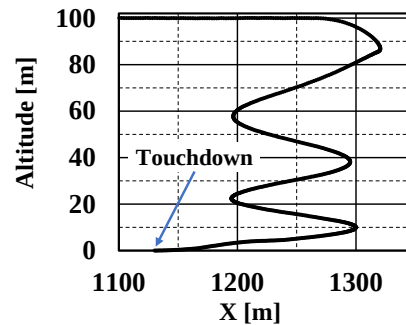
Fig.7(b) Flight path (X-Altitude).
