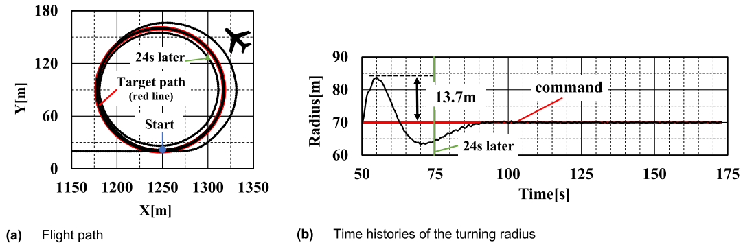
Fig.7 Simulation results (no wind).
