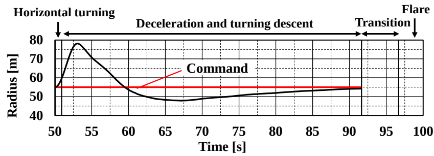
Fig.7(e) Time history of turning radius.
