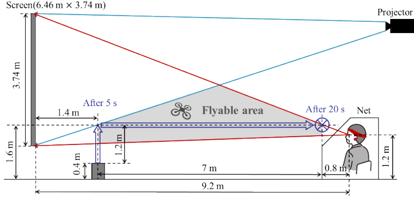
Fig.6 Flight path.
