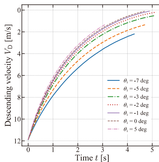
Fig. 11 Descending velocities (phase 2) ( \theta_a = 21 deg).
